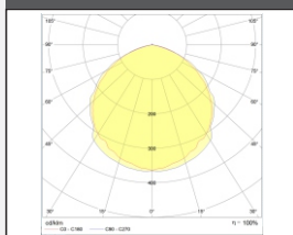
POLAR CURVE
